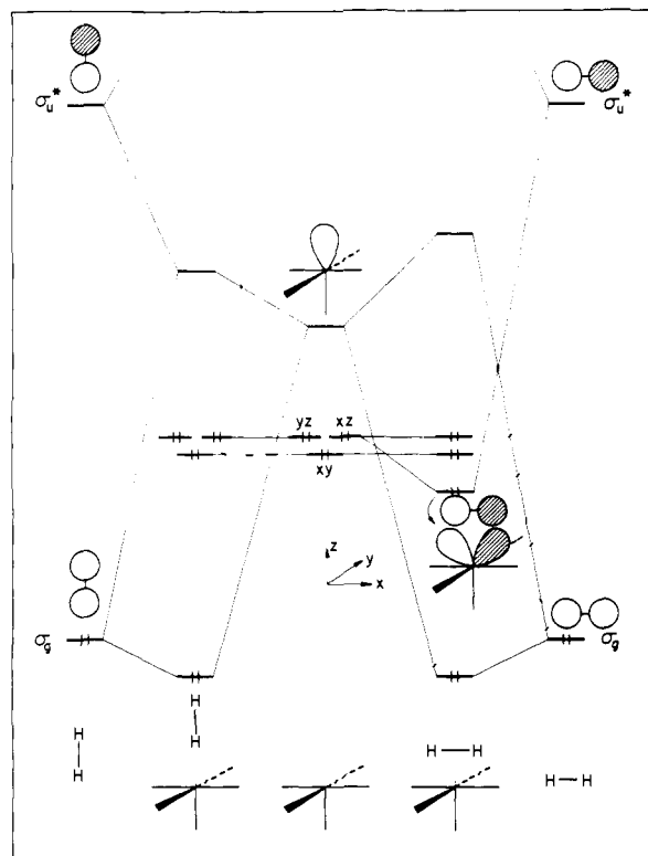
Figure 3. Interaction diagram for H 2 and Cr(CO) 5 for a perpendicular (left) and parallel (right) approach. The diagram is schematic in the position of the σ g and σ u * levels before and after interaction.
