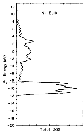
Figure 9. Density of states of bulk Ni.
