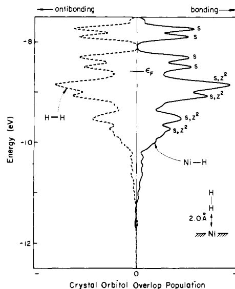
Figure 18. The COOP curve for Ni-H and H-H bonding in the d block region. H_2 here has approached to L = 2.0 \text{ \AA} . Those peaks in the COOP curve which pick up maxima in the projected DOS curve of surface s and z^2 are marked accordingly.
