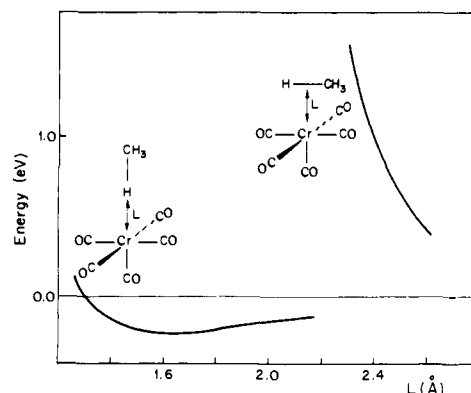
Figure 4. Total energy for perpendicular and parallel approaches of CH_4 to Cr(CO)_5 . The common energy zero for both curves is for both fragments at infinite separation.
