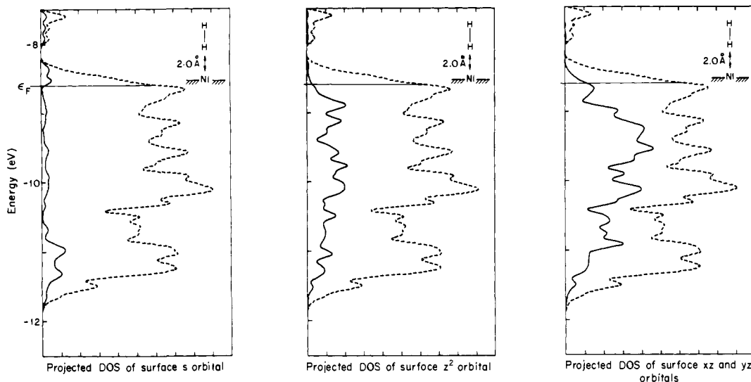
Figure 19. The parts of the total DOS of a four-layer slab model Ni(111) which are in the surface layers s , z^2 and xz , yz orbitals. The total DOS is represented, at a smaller scale, by the dashed line curve.
