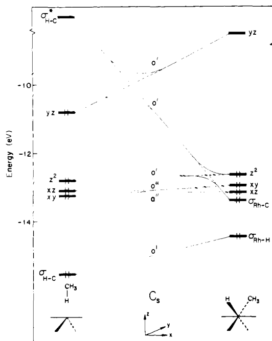
Figure 8. The evolution of the important energy levels along the oxidative addition reaction coordinate for \text{Rh}(\text{CO})_4^+ and \text{CH}_4 .
