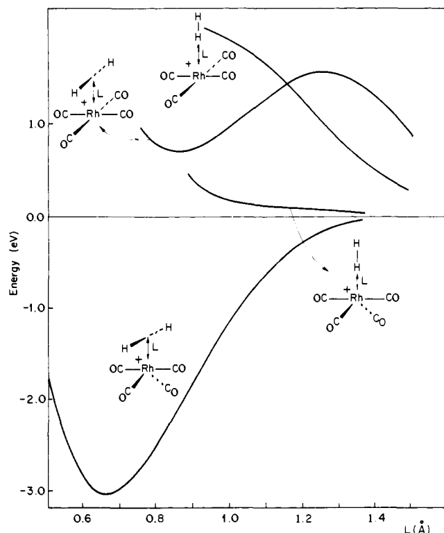
Figure 6. Total energy for perpendicular and parallel approaches of H_2 to a square-planar and angular Rh(CO)_4^+ . The common energy zero for all curves is at infinite separation of the fragments.
