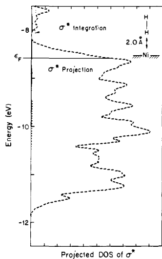
Figure 17. That part of the total DOS (dashed line) which is the H_2 \sigma^* (solid line hugging the energy axis). This is at L = 2.0 \text{ \AA} , and the energy window shows the Ni(111) d block only. The integrated \sigma^* population is the dotted line.
